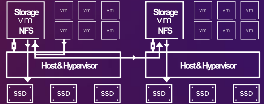
Committing a Write I/O in other HCI solutions
