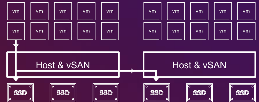
Committing a Write I/O in vSAN
