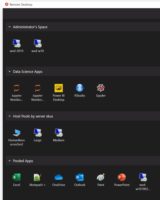
RD Client
